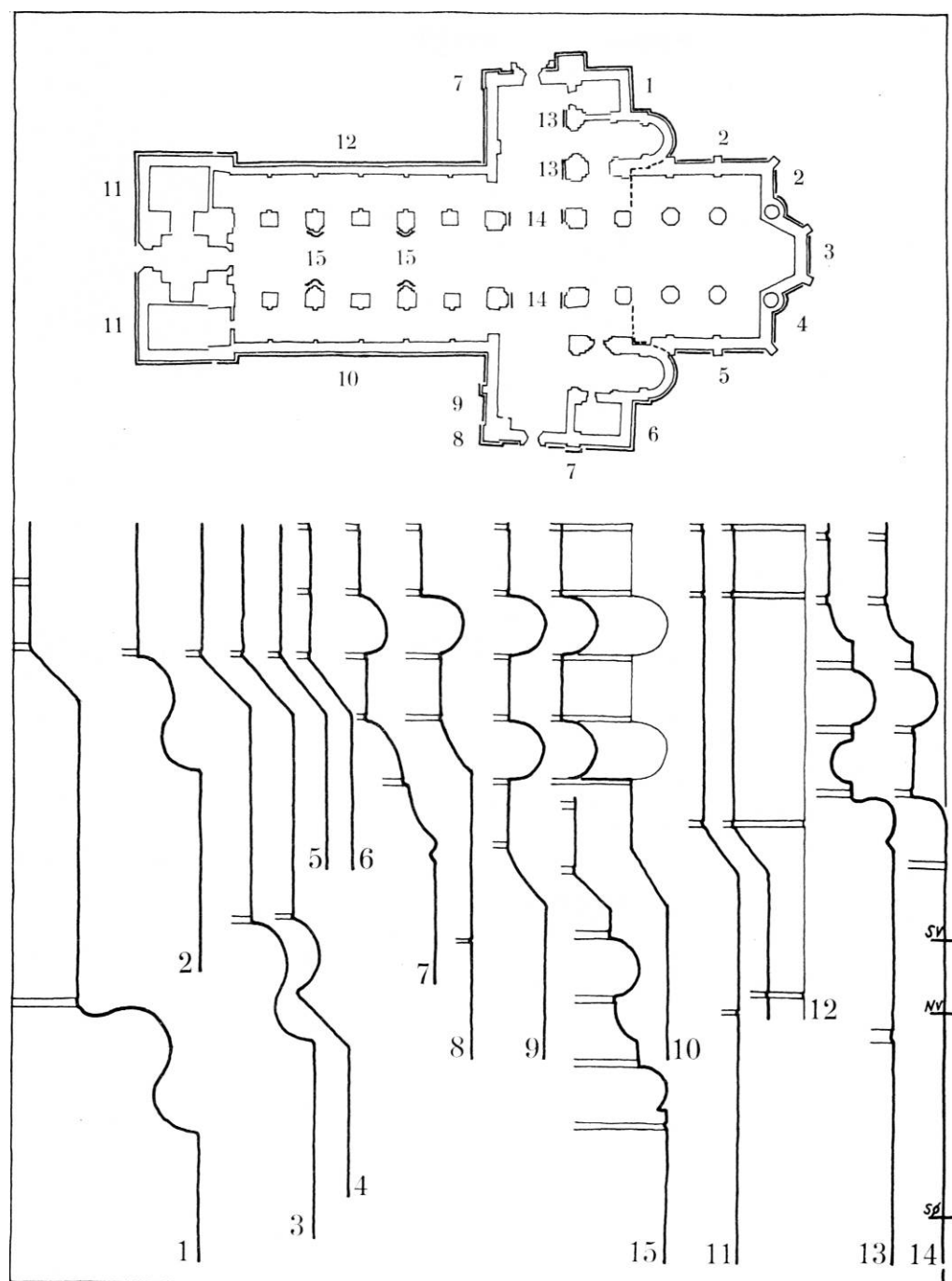
Fig. 31. Sokkeltyper 1:10, KdeFL (p. 131). — Types of plinth 1:10.
