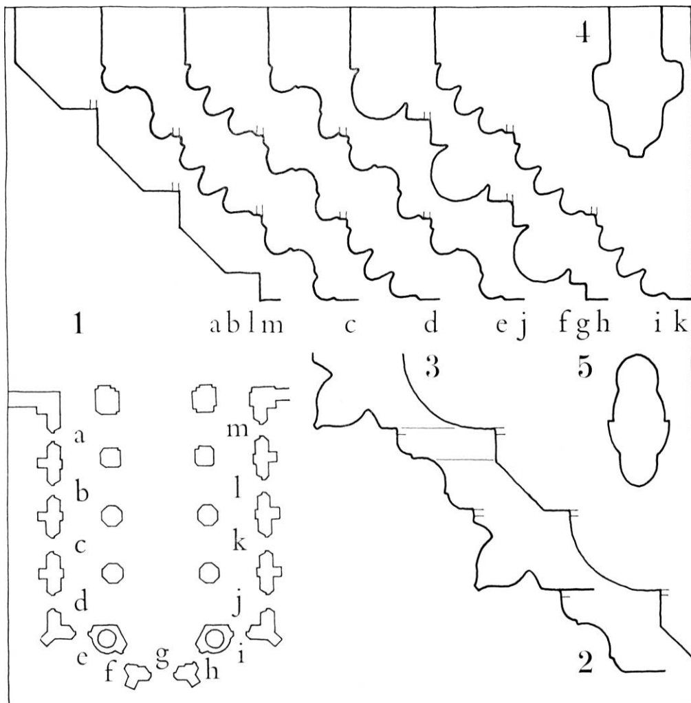
Fig. 132. Forskellige enkeltheder 1:10, KdeFL. 1. a-m. Korvinduernes profiler (p. 272). 2. Profiltype i vestportal, store vestvindue og højkirkevinduer (p. 233, 244). 3. Vinduesprofiltype i vestkapeller og nederste skifter i de fire vestre vinduer i højkirkens sydside (p. 224 og 244). 4. Løstliggende ribbesten, måske fra sideskibshvælv (p. 247). 5. Løstliggende stavværkssten fra vestkapel (p. 222). — Various details 1:10: 1. a m. The mouldings of the choir windows. 2. Type of moulding in west portal, large west window and nave windows. 3. Type of moulding in the windows in the west chapels and lowest courses in the four west windows on the south side of the nave. 4. Ribbing brick, possibly from the vaulting of side aisles. 6. Tracery brick from the west chapels.
