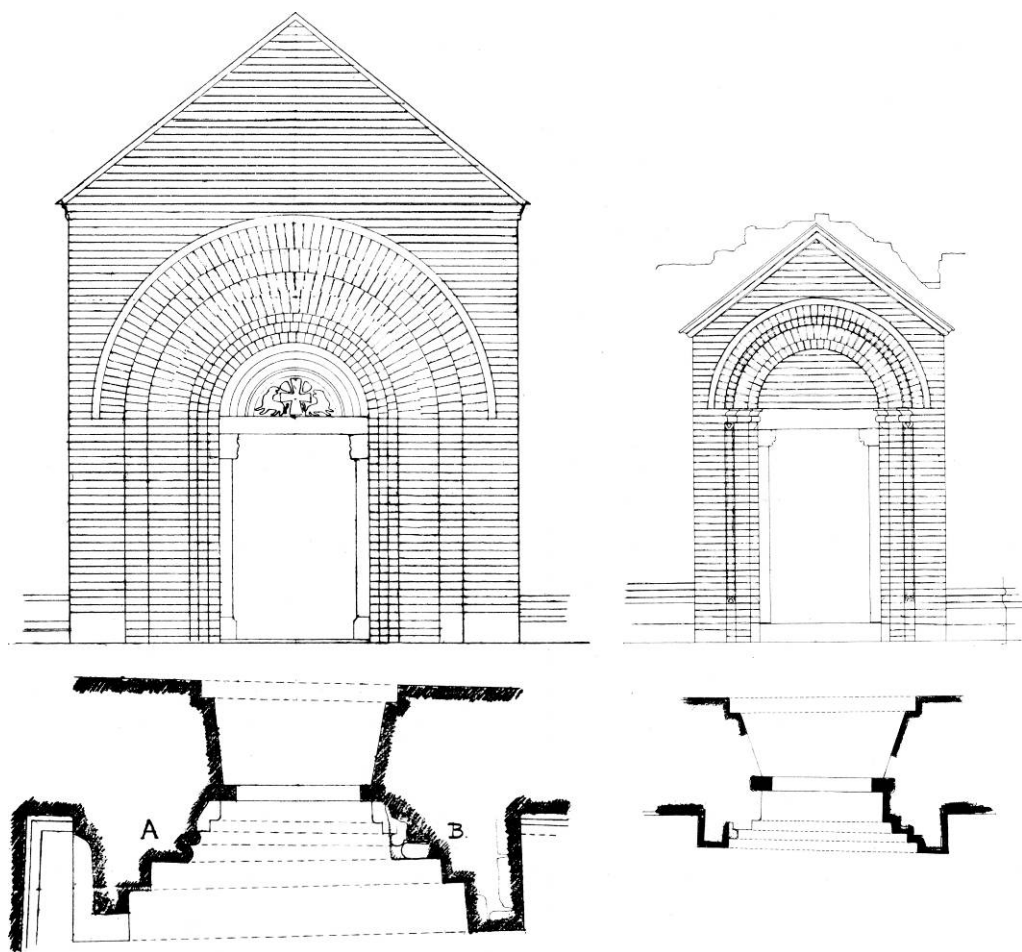
Fig. 166. Tværskibets portaler 1:100, t.v. nordportalen (1925), t.h. sydportalen (1922). Tegninger i NM af Mogens Clemmensen med angivelse af de partier, som Clemmensen anså for oprindelige, samt forslag til genopførelse. — The portals of the transept 1:100. To the left the north portal, to the right the south portal. The drawings were by Mogens Clemmensen during restoration in the 1920's, with indication of the parts which Clemmensen regarded as original, with suggestion for re-erection.
