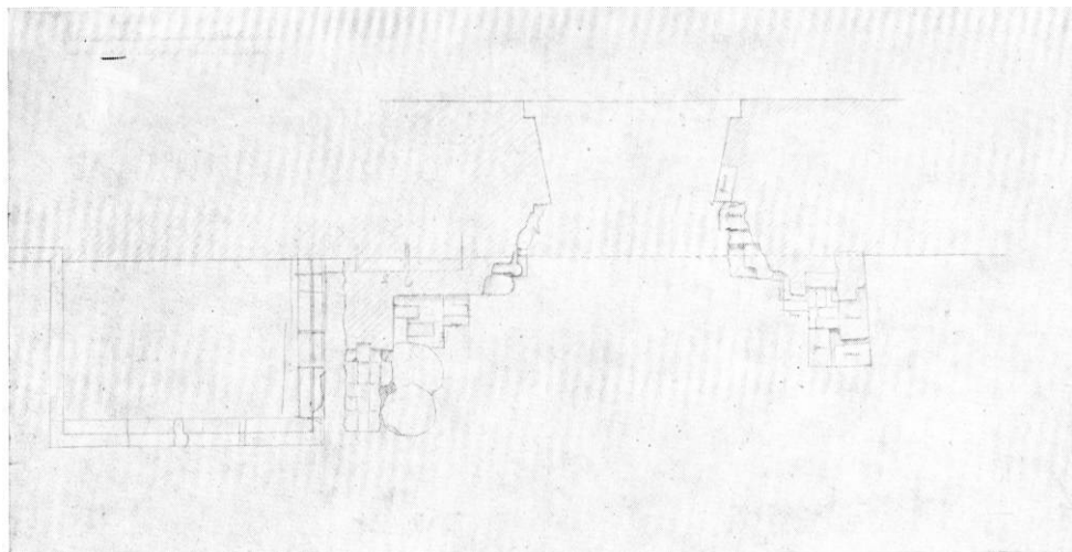
Fig. 53. Nordre korsarms portal, plan 1:100. Opmåling i NM af ældre fundamenter m.v., fremdraget ved ombygningen omkring 1X80 (p. 157). — Portal of the north transept, scale 1:100. Survey of older foundations etc., brought to light during the rebuilding c. 1880.
