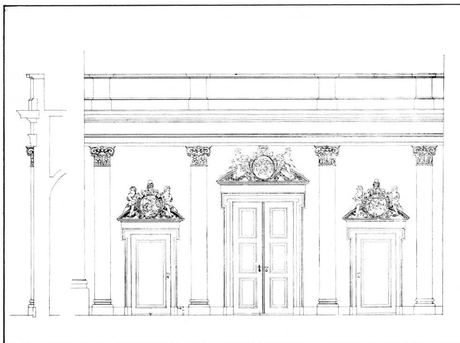
Fig. 167. Forsiden af det murede pulpitur i søndre korsarm 1:100. Mogens Clemmensens bygnings-tegning 1921. I domkirken. — Front of the masonry pulpitum in the south transept 1:100. Drawing for the erection 1921.
