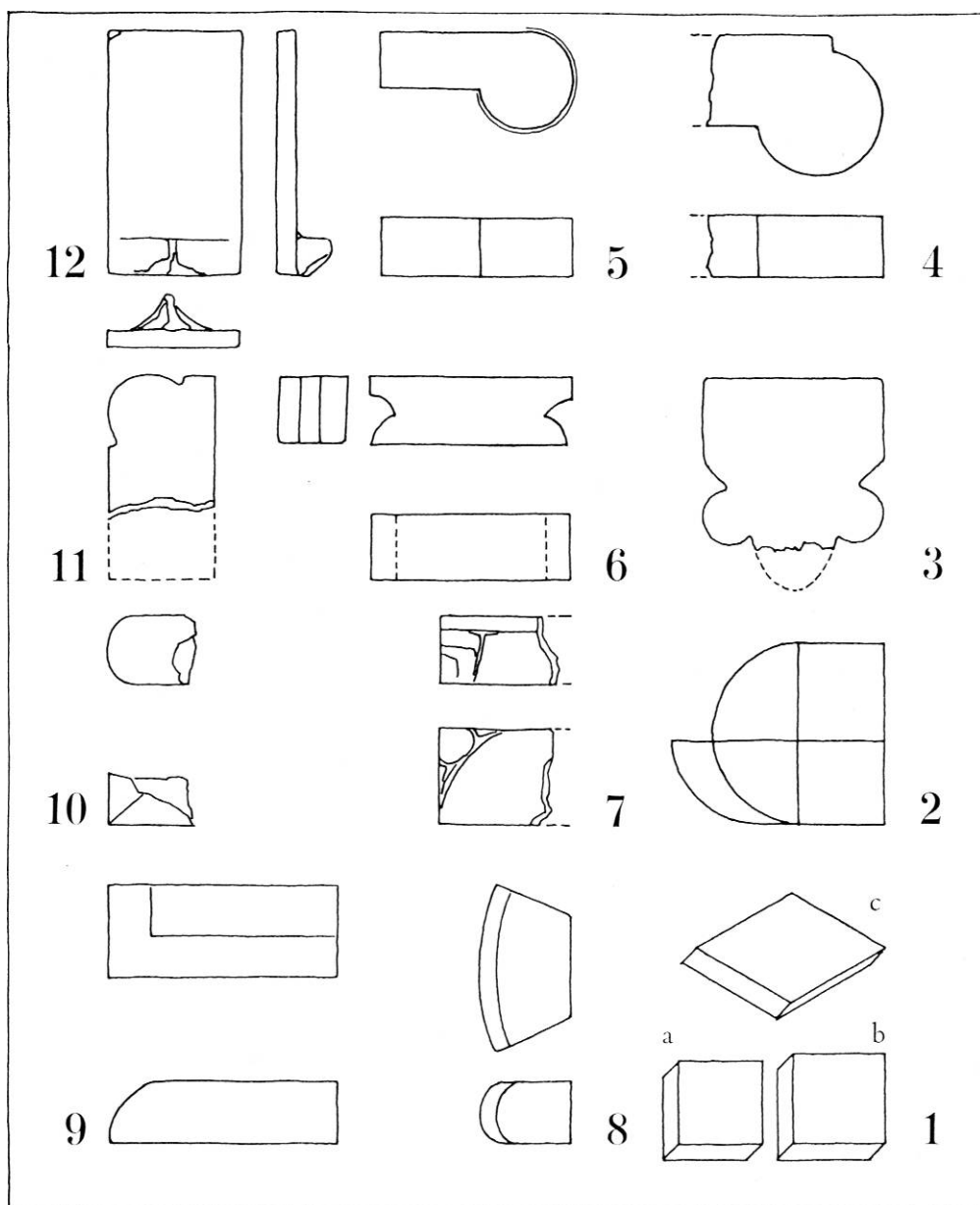
Fig. 174. Gulvfliser og formsten af rød tegl, løstliggende i kirkens stensamling på øverste galleri i nordre korsarm 1:10. KdeFL. 1. Gulvfliser, a. lys tegl, b. brunglaseret, c. gul- eller grønglaseret. 2. Tre, sikkert samhørende halvøjlesten. 3. Ribbesten. 4. Rundstav. 5. Rundstav, sort- eller grønglaseret. 6. Formsten. 7. Grønglaseret hjørneknop. 8. Søjlevulst. 9. Hjørneste. 10. Grønglaseret hjørneste. 11. Hjørneste. 12. Rektangulær tagpanne. — Floor tiles and mouldings of red brick to be found in the church's collection of building material in the top gallery in the north transept 1:10. 1. Floor tiles, a. light coloured brick, b. brown glazed, c. yellow or green glazed. 2. Three bricks, no doubt belonging together, from an engaged column. 3. Rib brick. 4. Billet. 5. Billet, black or green glazed. 6. Moulded brick. 7. Green glazed corner boss. 8. Torus. 9. Cornerstone. 10. Green glazed cornerstone. 11. Corner fillet. 12. Rectangular pantile.
