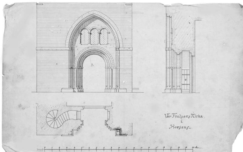
Fig. 79. Plan, opstalt og snit af hovedportal mod Torvet, tegnet af H. B. Storck 1880 (s. 5466). Udateret kalke ved Hector Estrup. 1:150. I Horsens Museum. – Plan, elevation and section of main portal towards the square Torvet, drawn by H. B. Storck 1880. Undated tracing by Hector Estrup.
