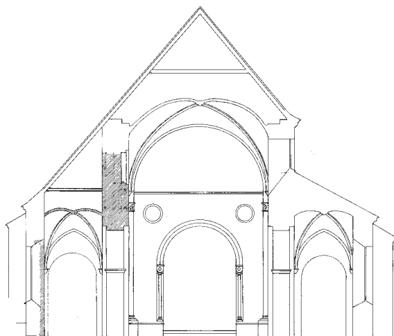
Fig. 81. Tværsnit i skibet mod øst. 1:300. Restaureringsprojekt med blyantsskitser af de under arbejdet fremkomne triforier. Viggo Norn 1935. I Horsens Museum. – Cross-section of the nave towards the east. Restoration project, 1935, with pencil sketches of the triforia that emerged during the work.
