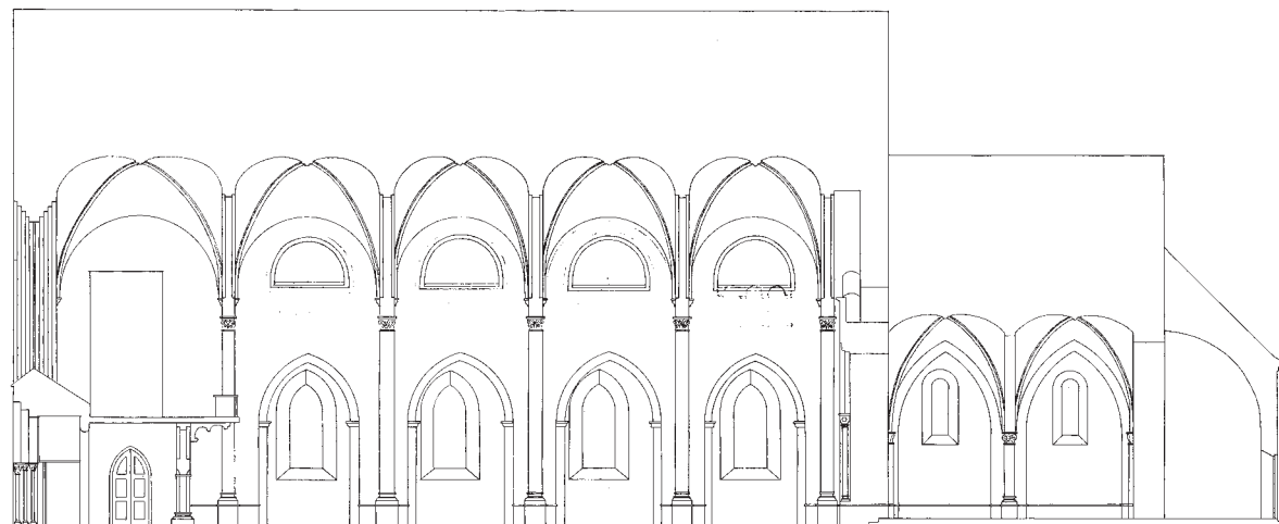
Fig. 83. Længdesnit mod nord. 1:300. Restaureringsprojekt med blyantsskitser af de under arbejdet fremkomne triforier. Tegnet af Viggo Norn 1935. I Horsens Museum. – Longitudinal section towards the north. Restoration project, 1935, with pencil sketches of the triforia that emerged during the work.
