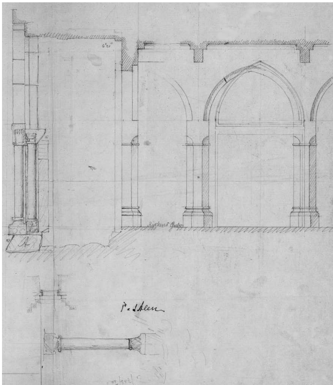
Fig. 39a-b. Plan og opstalt af vestportal (s. 5411), tegnet af Hector Estrup under restaureringen 1879-81. 1:50. I Horsens Museum. – Plan and elevation of west portal, drawn by Hector Estrup during the restoration in 1879-81.
