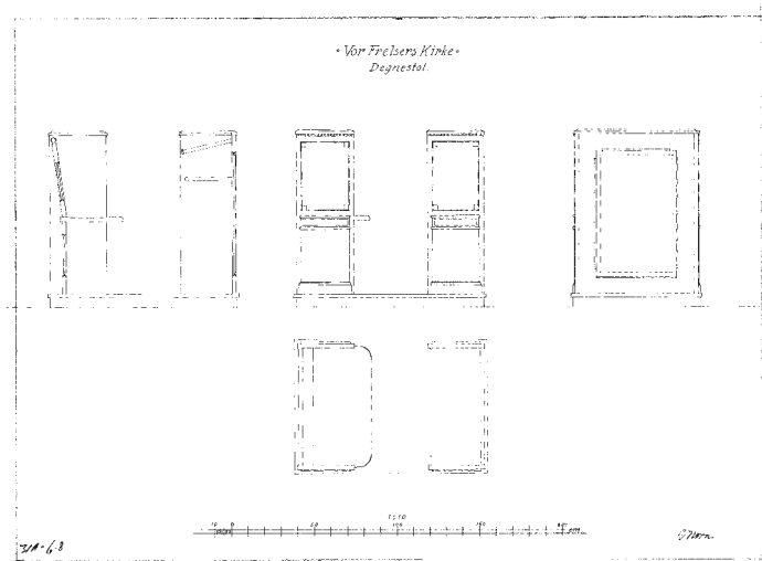
Fig. 151. Udkast til degnestol, 1935-36 (s. 5333). 1:50. Tegning af Viggo Norn. I Horsens Museum. — Proposal for chair for the parish clerk, 1935-36. Drawing by Viggo Norn.
