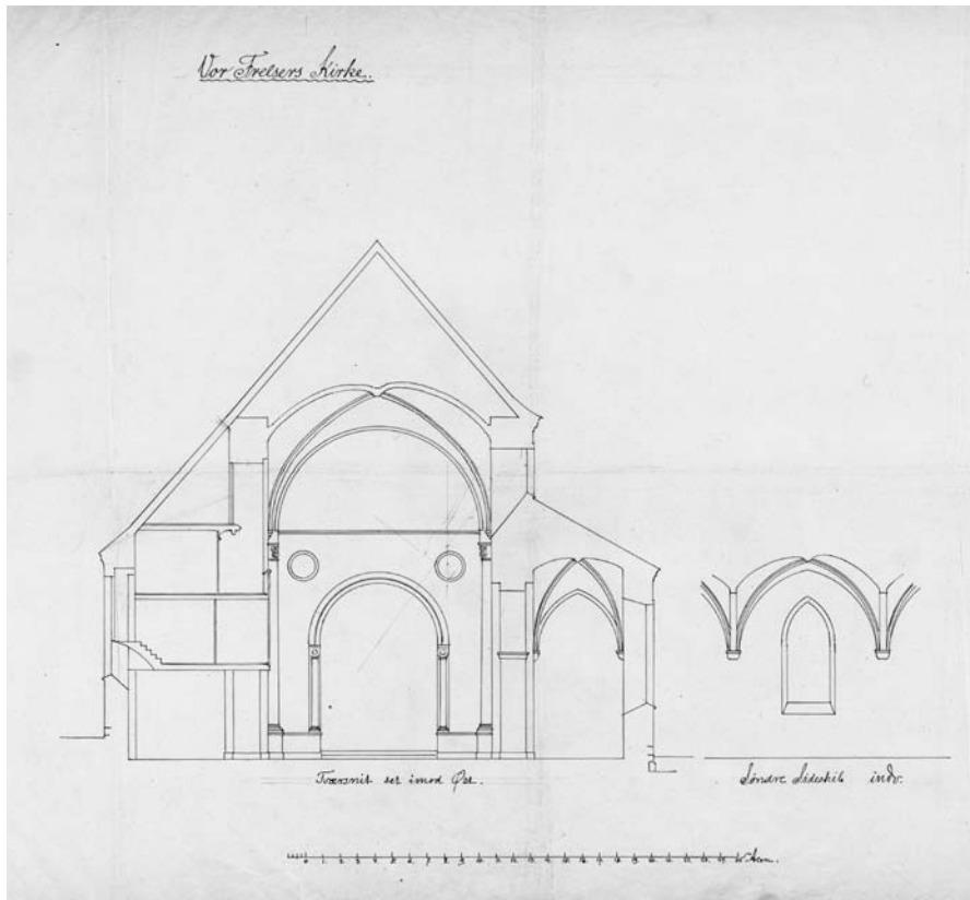
Fig. 76. Snit af skibet set mod øst efter V.Th. Walthers restaurering 1864-66. Opmåling ved Hector Estrup 1879. 1:300. – Cross-section of the nave towards the east, 1879, after the restoration by V.Th. Walther 1864-66.
