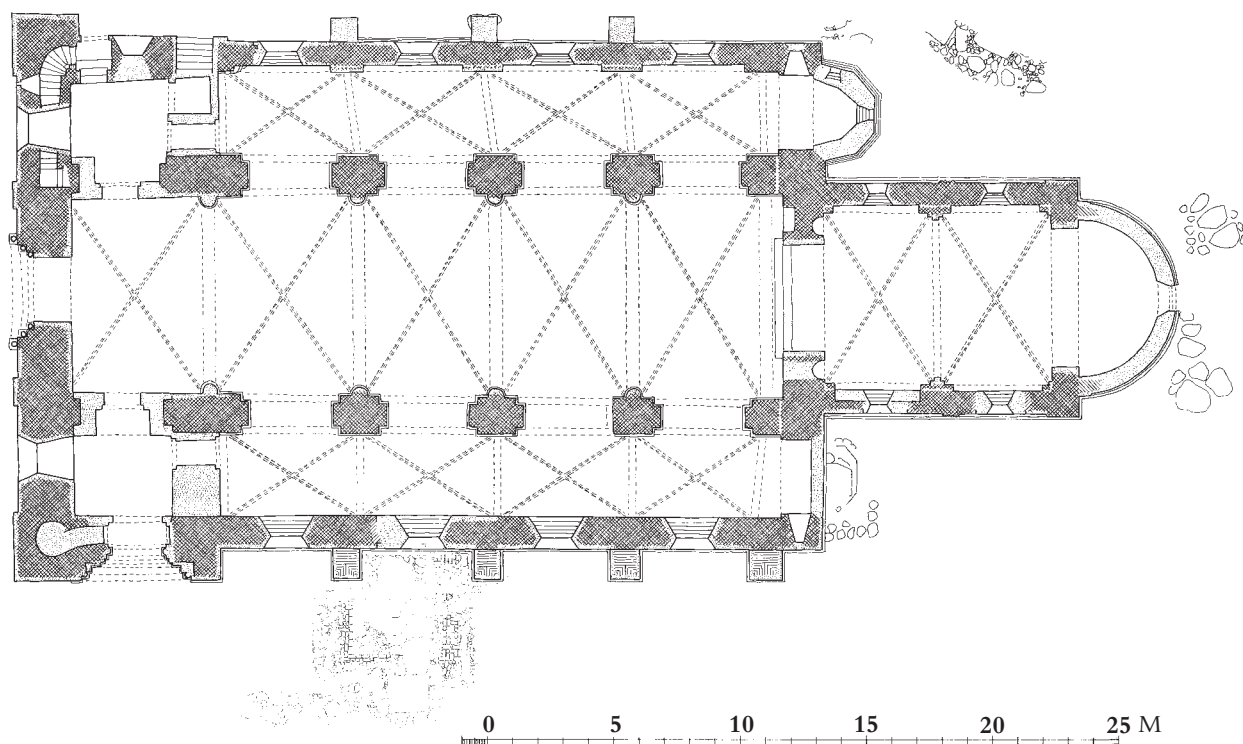
Fig. 28. Plan. 1:300. Målt af Viggo Norn 1935-36; fundamenter øst for kirken målt af Hector Estrup 1879-80 og Horsens Museum 1991. Tegnet af Mogens Vedsø 2004. Fundamentet af \ddot{t} våbenhus syd for kirken tegnet af Ina D. Holst 1993 efter opmålinger i Horsens Museum 1992. Signaturforklaring s. 10. – Ground plan. 1:300. Measured by Viggo Norn 1935-36; foundations east of the church measured by Hector Estrup in 1879-80 and by Horsens Museum in 1991. Drawn by Mogens Vedsø, 2004. Foundations of \ddot{t} porch south of the church drawn by Ina D. Holst 1993 after measurements in Horsens Museum, 1992. Key on p. 10.
