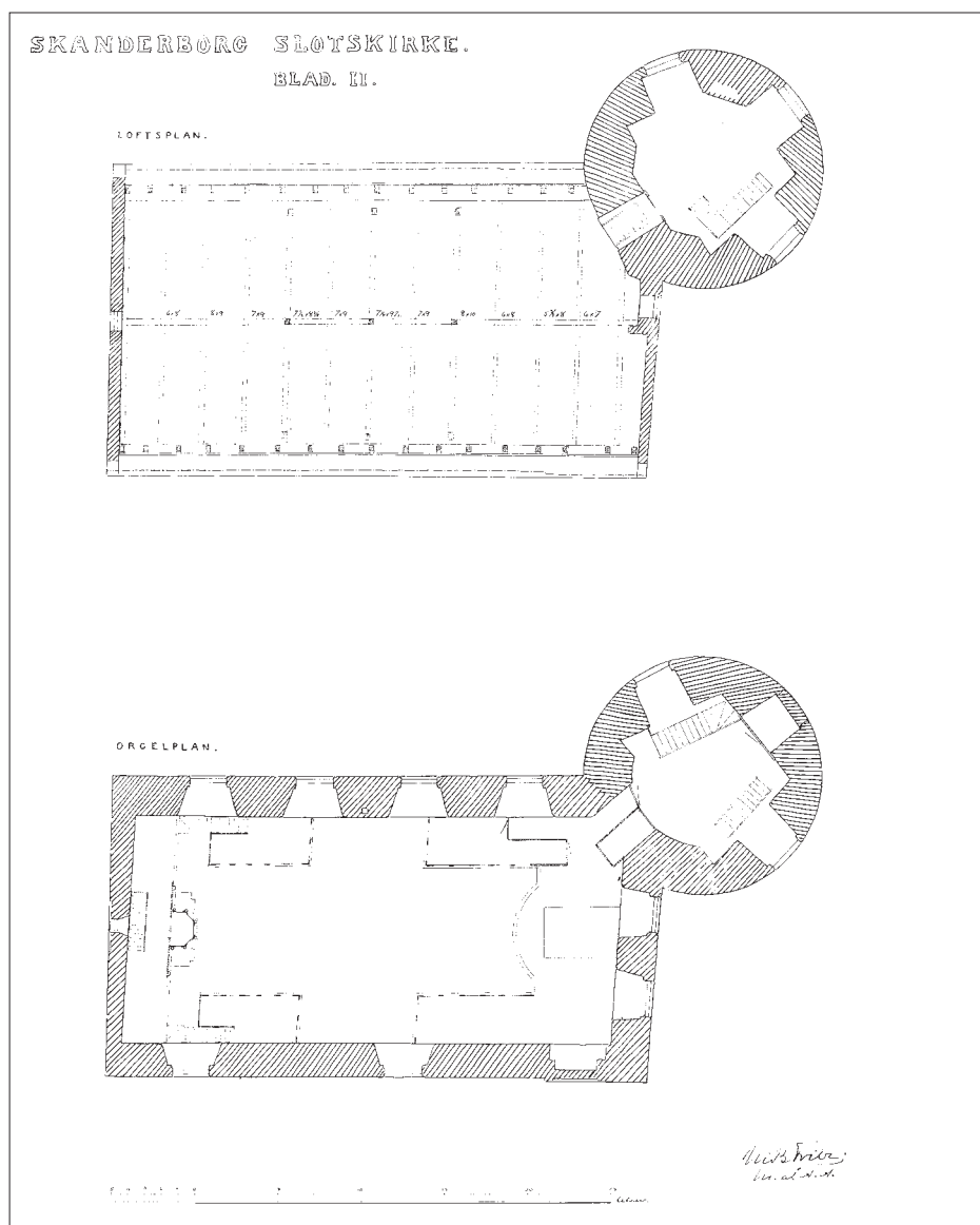
Fig. 24d-e. Planer af kirkens loft og pulpituretage. Tegnet af M. B. Fritz 1909. — Plans of the church loft and gallery floor.
