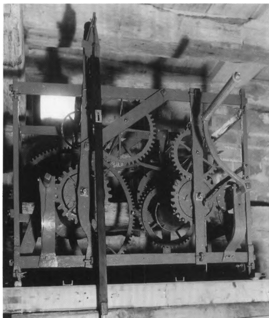
Fig. 45a-b. Tårnur, formodentlig fra 1700'rne. a. Helhed. b. Jernstemplers (s. 2234). HS fot. 1990. - a-b. Tower clock, probably 18th century. a. In its entirety. b. Marks.
