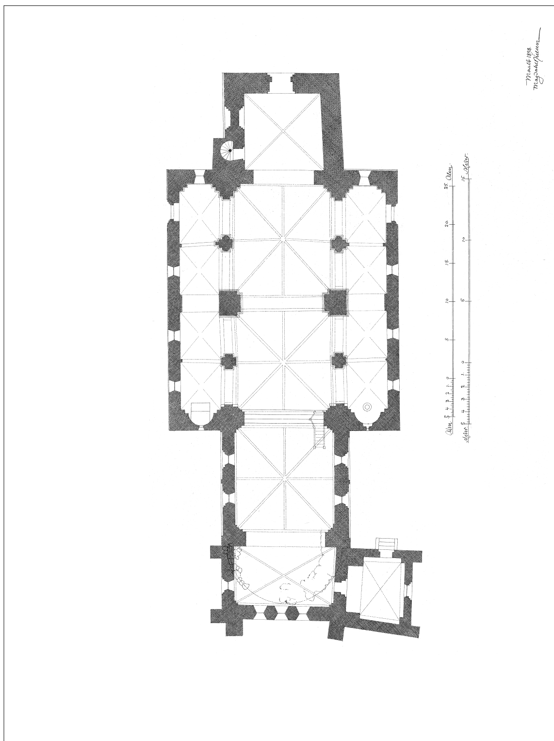
Fig. 22. Grundplan med apsisfundamenter fremkommet under restaureringen 1892-94. 1:300. Vest opad. Opmåling ved J. Magdahl Nielsen 1898. – Groundplan with the foundations of the apse exposed during restoration in 1892-94. West at top.
