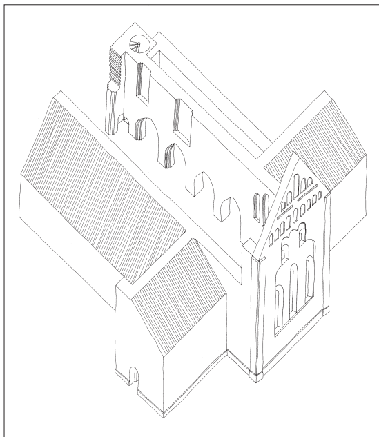
Fig. 46. Rekonstruktion af kirkens 3. byggefase, 1275–1300, set fra sydøst. 1:600. Tegnet af Pia K. Lindholt 2022. – Reconstruction of the third construction phase of the church, 1275–1300, seen from the south east.
