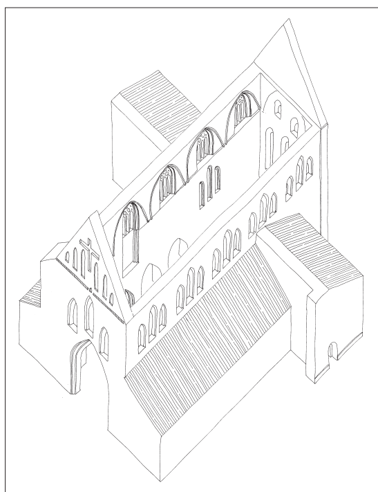
Fig. 58. Rekonstruktion af kirkens 5. byggefase, 1300-50, set fra sydvest. 1:600. Tegnet af Pia K. Lindholt 2022. – Reconstruction of the fifth construction phase of the church, 1300-50, seen from the south west.
