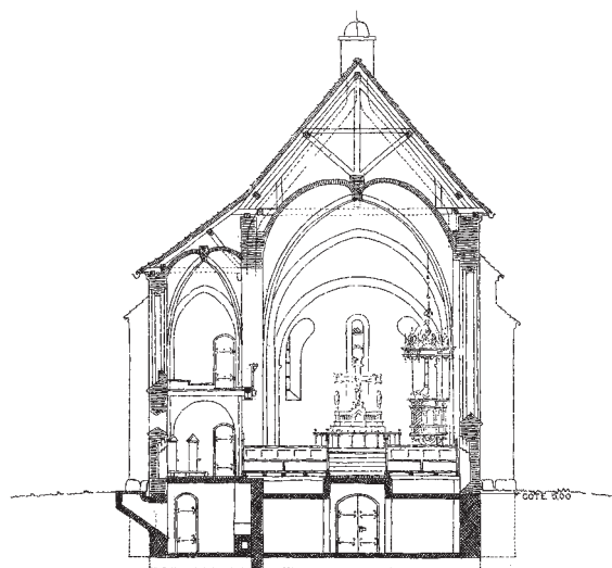
Fig. 8. Tværsnit set mod øst. 1:300. H. Lønborg-Jensen 1938. — Cross-section viewed towards the east.
