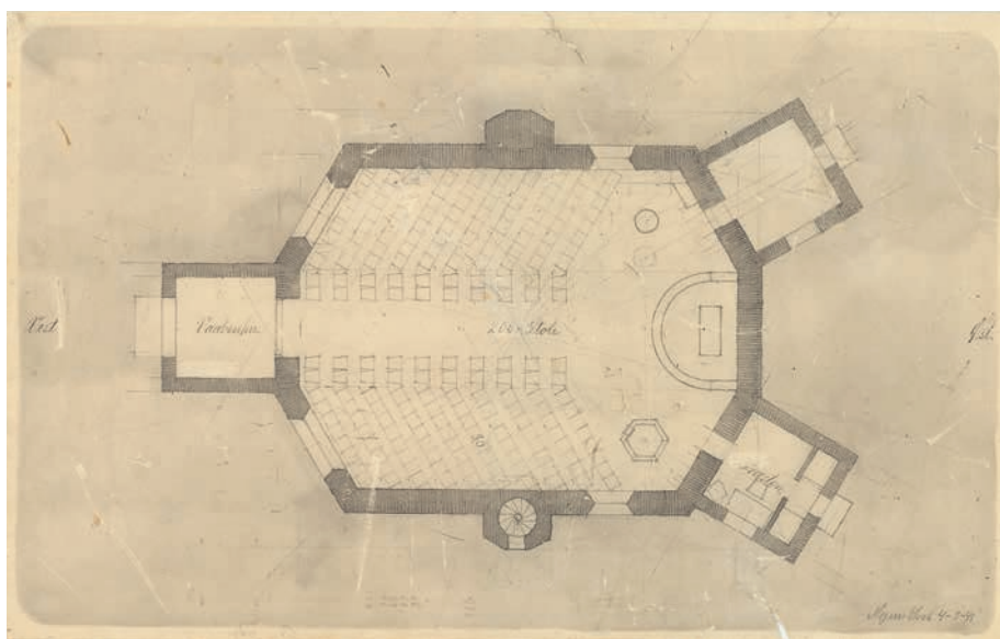
Fig. 5. Forstudie. 1:500. Skitse ved Mogens Koch 1941. Mogens Koch Design I/S. – Preliminary study.
