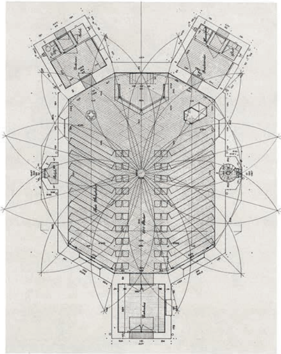
Fig. 21b–c. Geometriske principper. 1:300. b. Plan. Efter Karlsen 1968. c. Gulyplan. Mogens Koch, udateret. Mogens Koch Design I/S. – Geometric principles. b. Plan. c. Floor plan.
