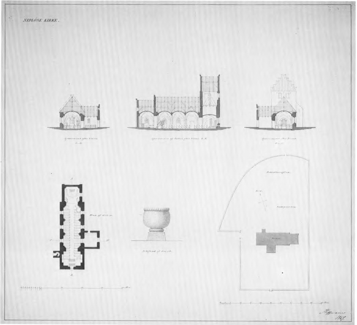
Fig. 13-14. To farvelagte blade med planer af kirkegård og kirke samt snit og opstalter, signeret »Hoffmann 1867«. Bygningstegneren Georg Hoffmann udførte tilsvarende sæt af de andre Akademikirker samt til Universitetets kirker. Tegningerne giver ofte værdifuld oplysning om tilstanden i 1860'erne, men er dog ikke fuldtud pålidelige i enkeltheder. — Two coloured leaves with plans of churchyard and church, as well as sections and elevations, signed by "Hoffmann 1867". The architectural draughtsman Georg Hoffmann made corresponding sets of the other Academy churches and of the churches belonging to the University. The drawings often give valuable information about the state of these churches in the 1860s, but are not always fully reliable in detail.
